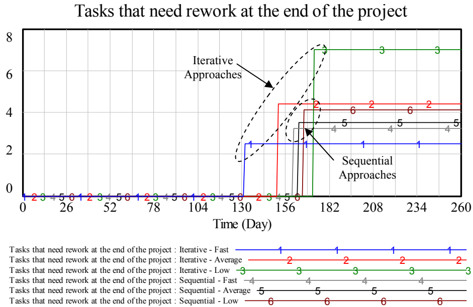
Figure 26. Insight evolution sensitivity.
