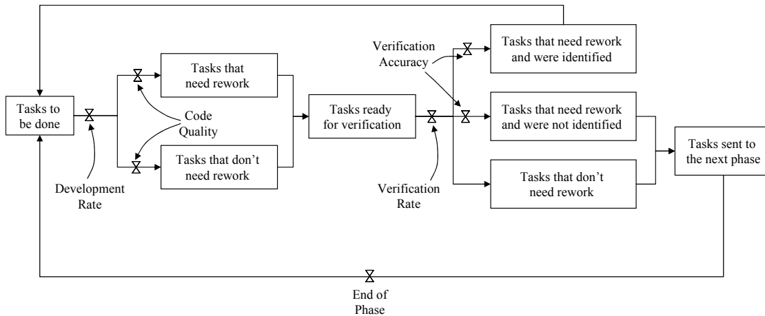
Figure 7. High level view of the Model.
